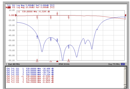
Insertion Loss(SS)
