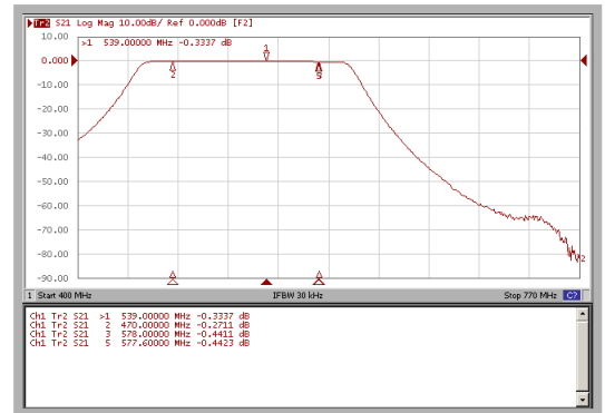
Insertion Loss(NS)
