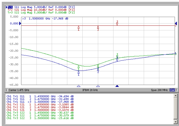
(L-Band 2Way Combiner)
