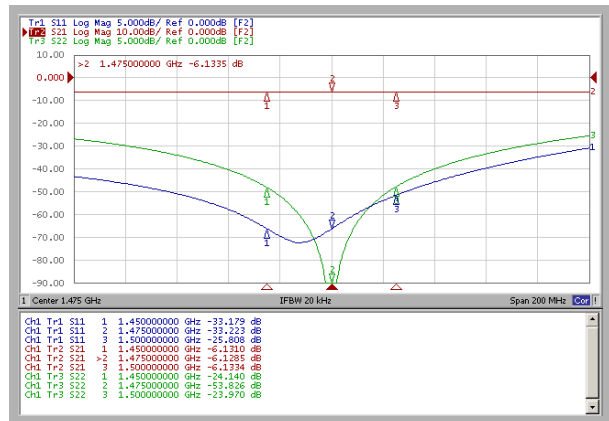
(L-Band 4Way Combiner)
